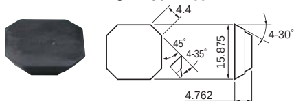
Fig.1 SGHN1504AZN-44
