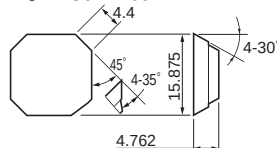
Fig.3 SGLN1504AZN-44
