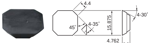
Fig.3 SGLN1504AZN-44
