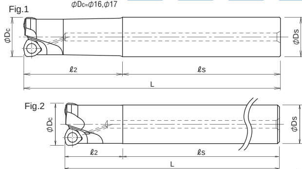
φDc=φ16, φ17
